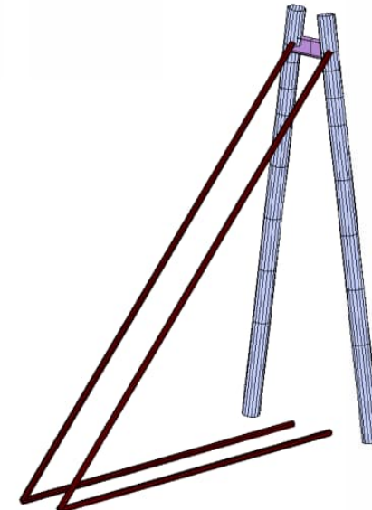
Figur 4-2: GTStrudl-model, isometri
